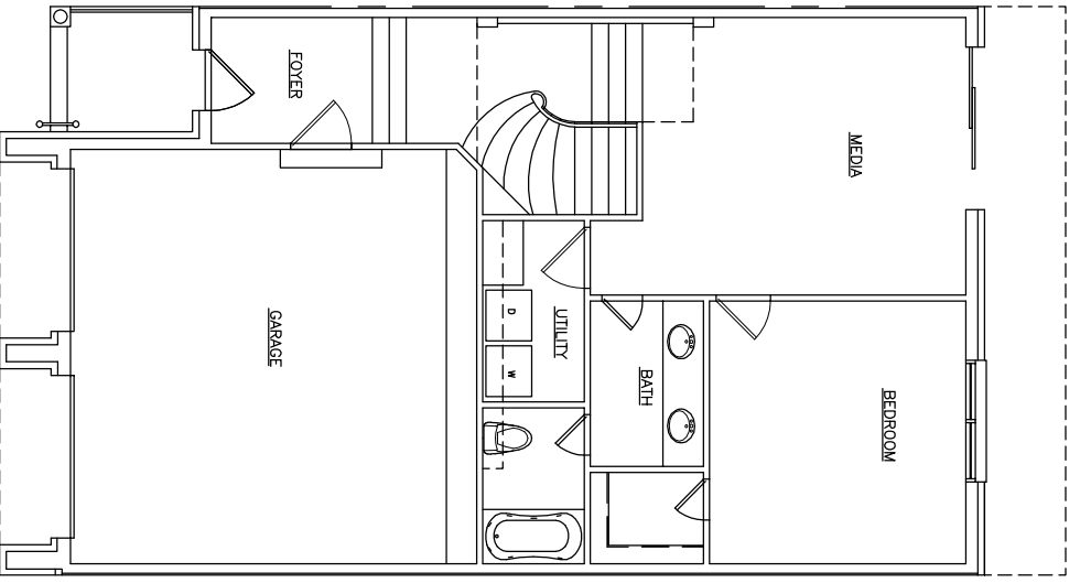
FIRST FLOOR OPTION 3 ONE BEDROOM/MEDIA
