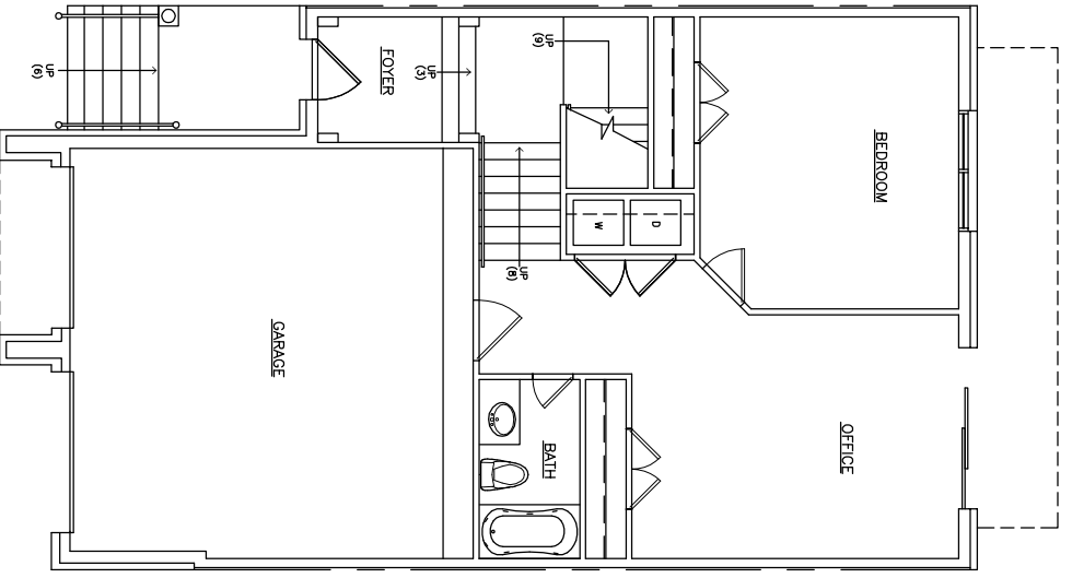
FIRST FLOOR OPTION 2 ONE BEDROOM/OFFICE
