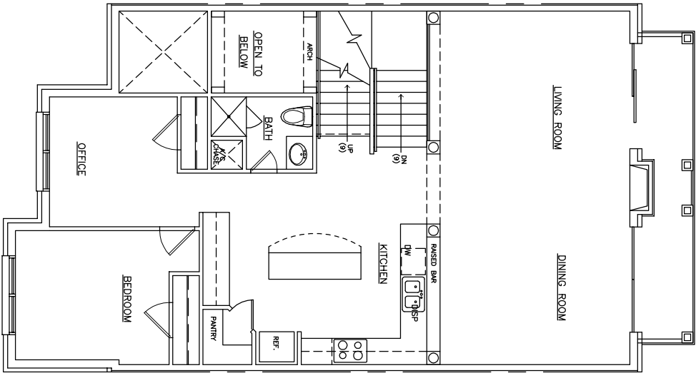
SECOND FLOOR OPTION 1 ONE BEDROOM/OFFICE
